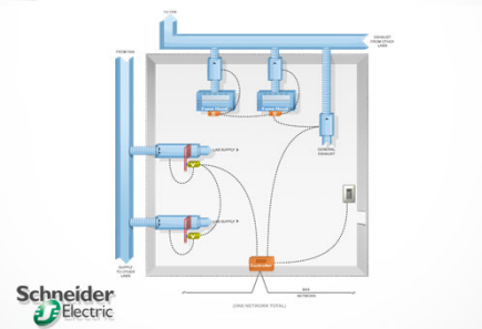
Laboratory Controls on BAS Native Controller
