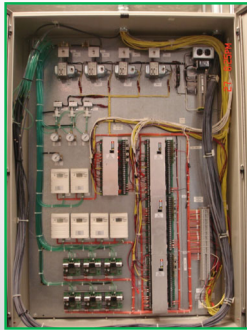
1 st Generation AHU Panel
